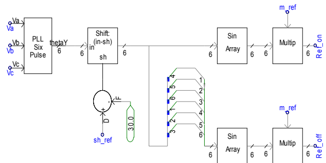
Fig. 6. Generating sine wave signal model.
