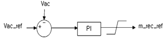
Fig. 9. AC voltage controller at rectifier.
