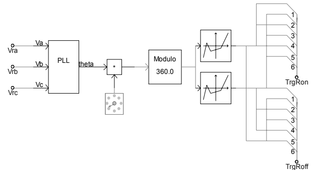
Fig. 5. Generating carrier signal model.
